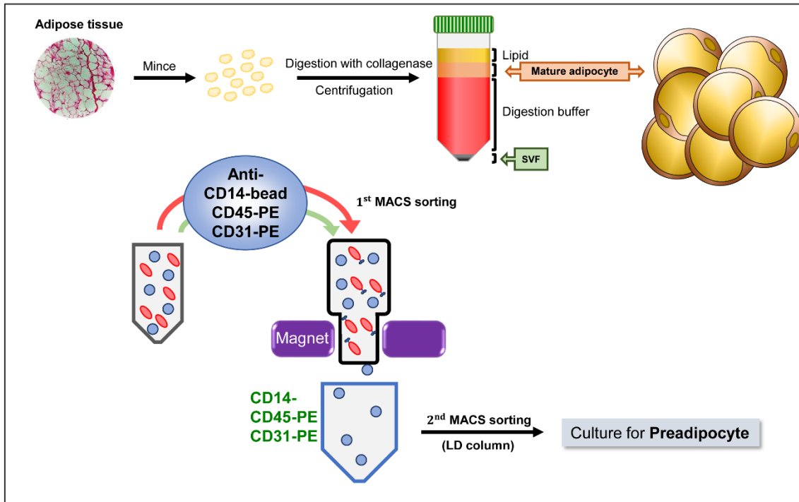
Figure S5. Schematic of purification of AC and preAC cells from AT.
